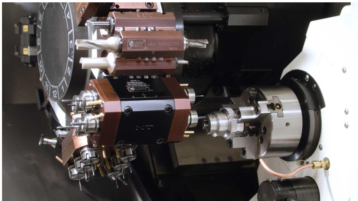
Multiple Output Driven Toolholder
